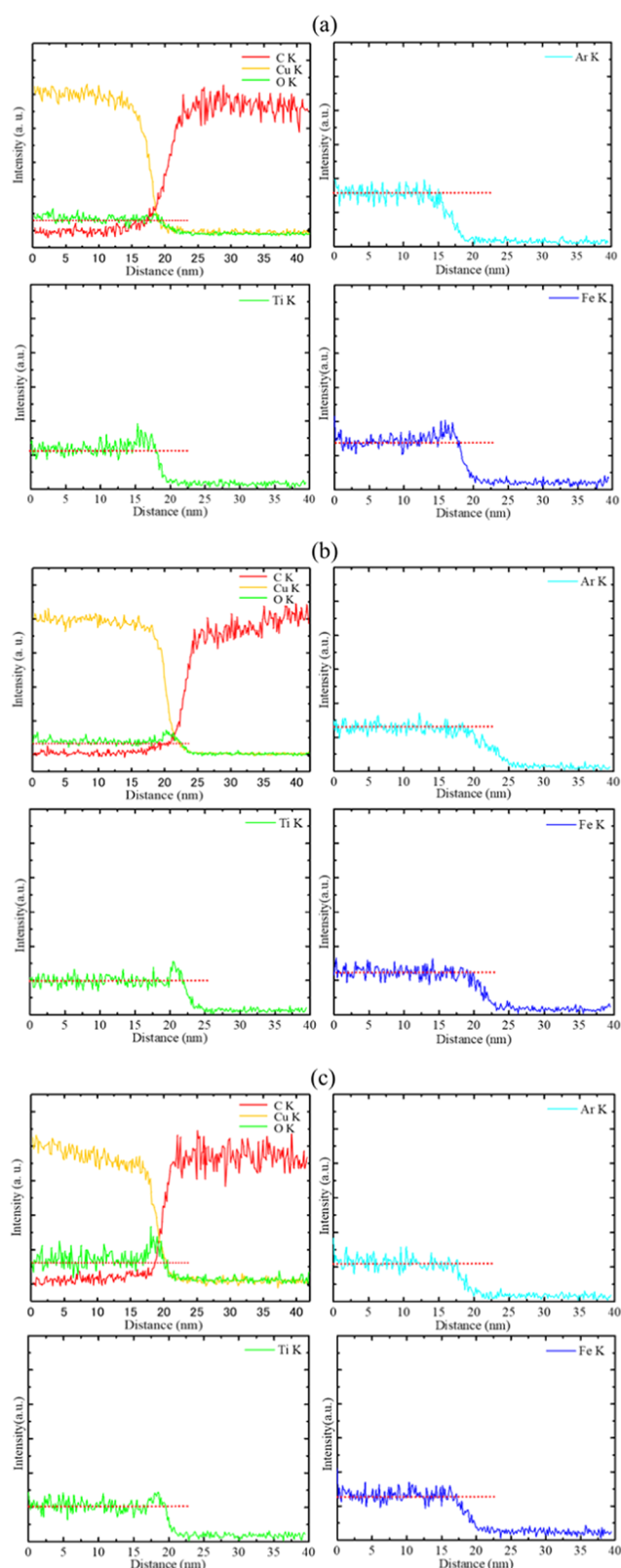
Figure 4. X-ray intensity profiles of C, Cu, O, Ar, Ti, and Fe in the as-bonded Cu/diamond interface (a) and the interfaces annealed at 500 °C (b) and 700 °C (c). The red dotted line shows the average intensity of the background noise.
