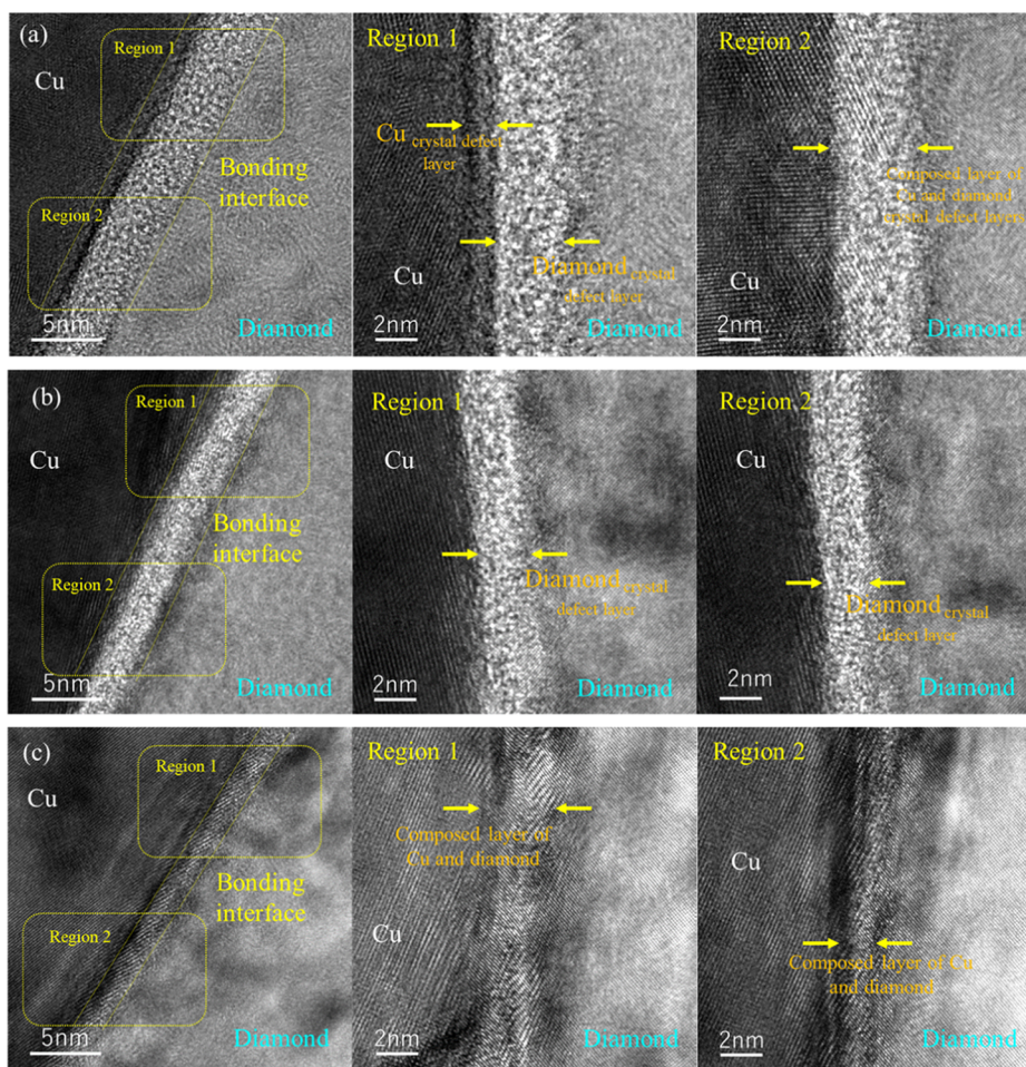
Figure 3. Cross-sectional STEM images of the as-bonded Cu/diamond interface (a) and the interfaces annealed at 500 °C (b) and 700 °C (c).
