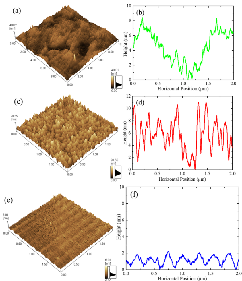
Figure 2. AFM images and corresponding cross-sectional profiles of the Cu plate (a, b), the deposited Cu thin film (c, d), and the diamond substrate (e, f) surfaces.
